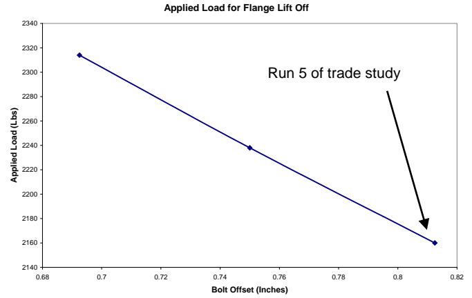
Figure 11 - Conventional Flange
